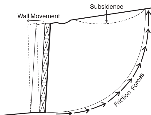
Figure 4 - Wall movement
