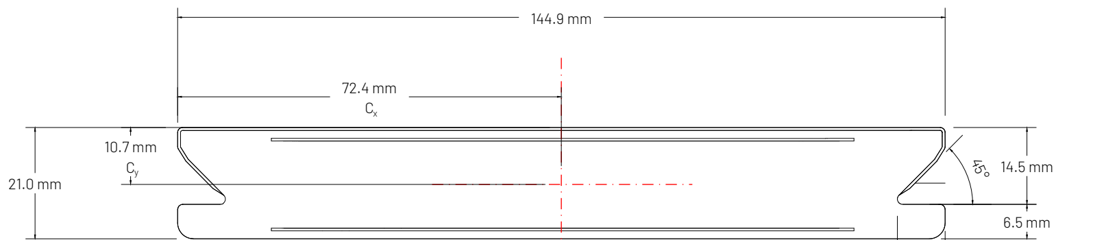
A STF101A Grooved deck board Scale 1:1
