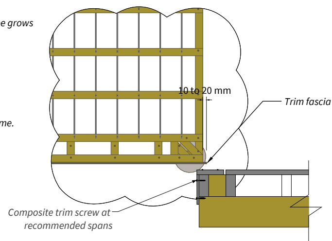
5 Trim detail
