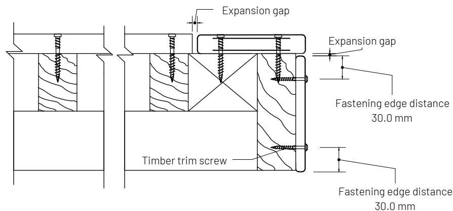
B1 STFM106. Grooved deck board in a Timber application beneath a breaker board Scale 1:5
