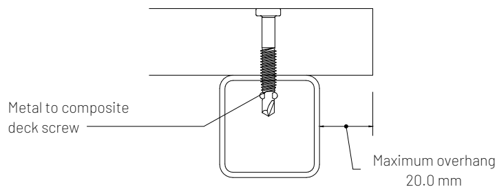
B2 STF102A- Square edge deck board in a metal application Scale 1:2
