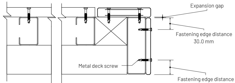
B1 STF106. Grooved deck board in a metal application beneath a breaker board Scale 1:2
