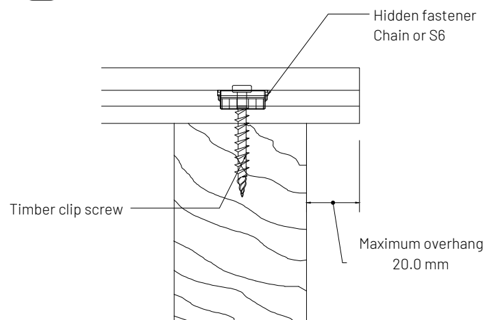
A STF101A Grooved deck board Scale 1:1
