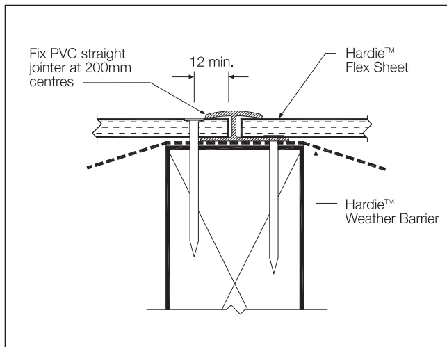
FIGURE 7 PVC STRAIGHT JOINER
