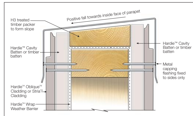
FIGURE 27 PARAPET DETAIL
