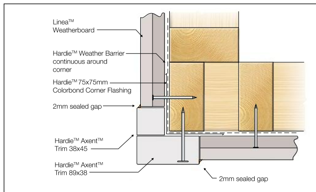
FIGURE 5 EXTERNAL CORNER TRIM OPTION
