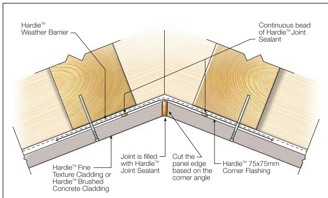
FIGURE 20 SEALANT FILL OPTION - LESS THAN 90° INTERNAL CNR
