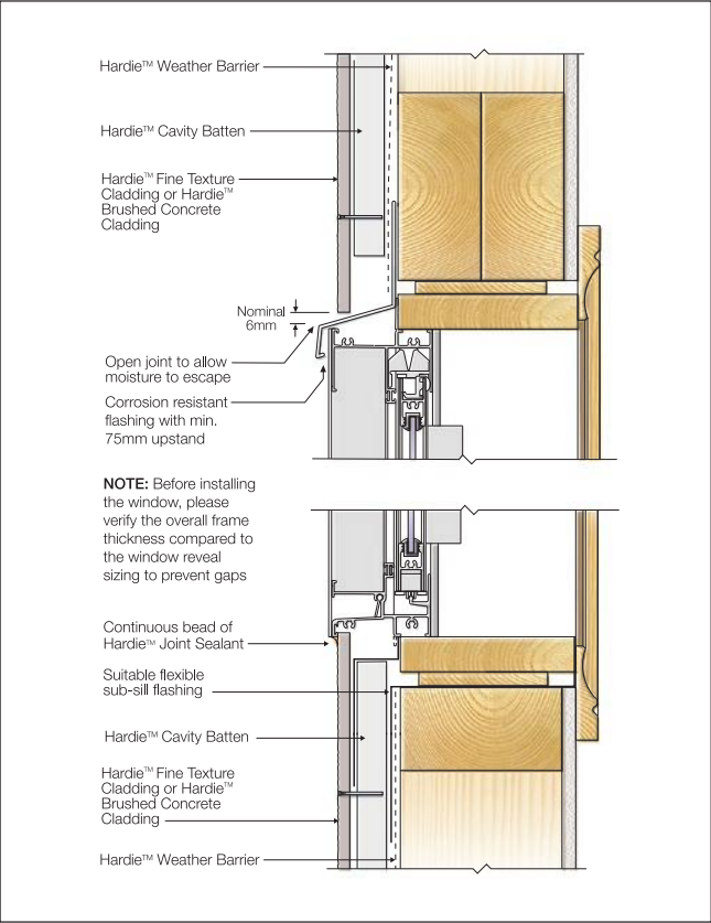
FIGURE 35 WINDOW HEAD AND SILL - CAVITY BATTEN
