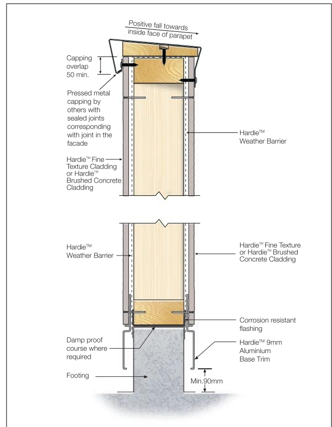
FIGURE 7 BLADE WALL
