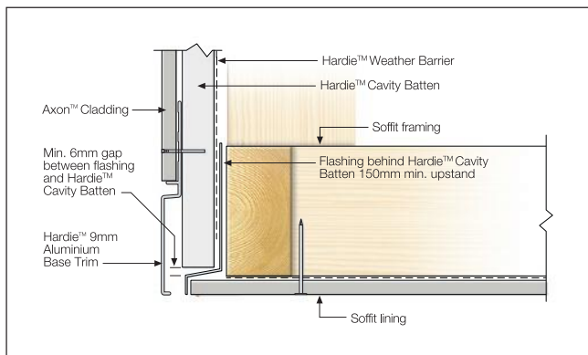
FIGURE 21 FACADE/SOFFIT JUNCTION
