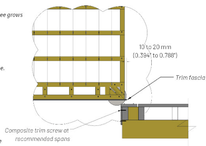
5 Trim detail
